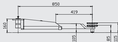
Short arm
